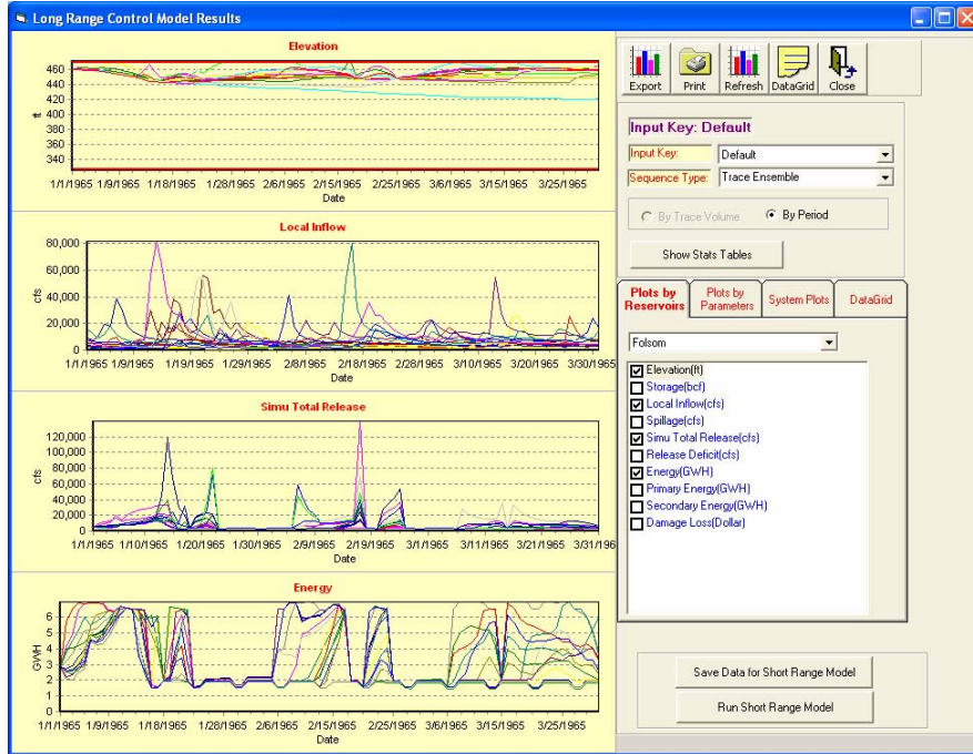
Figure H-1: Example Elevation, Inflow, Release, and Energy Sequences; Folsom
