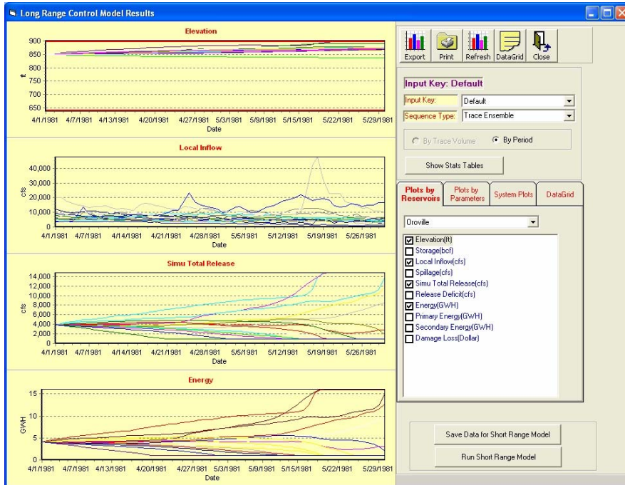
Figure H-2: Example Elevation, Inflow, Release, and Energy Sequences; Oroville
