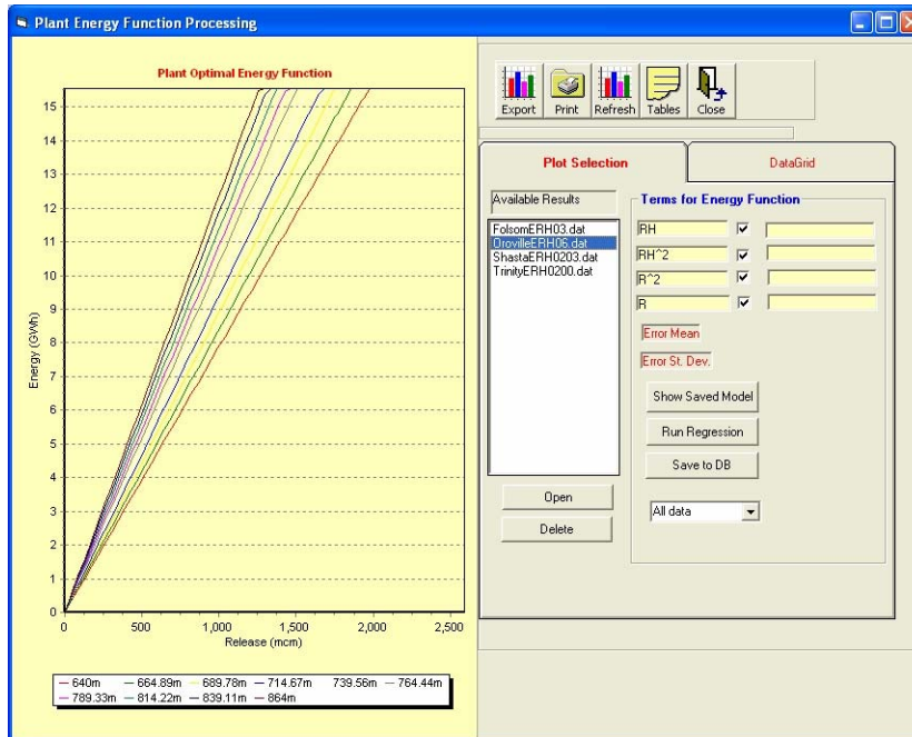
Figure G-2: Daily Energy Generation Function; Oroville
