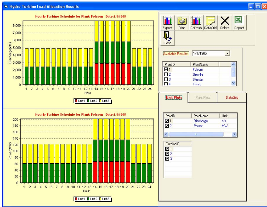
Figure G-3: Example Daily Discharge and Generation Sequences; Folsom
