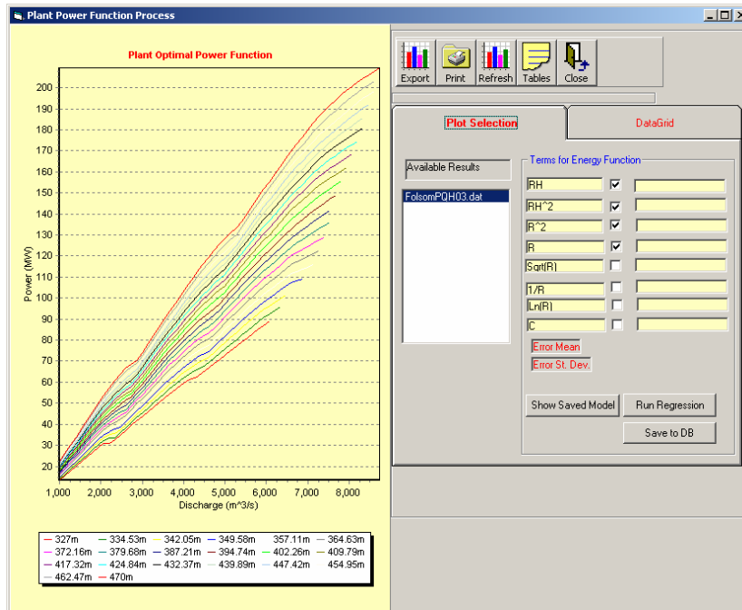
Figure F-2: Best Efficiency Plant Generation Curves; Folsom
