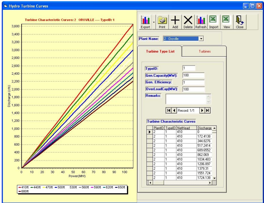
Figure F-3: Oroville Turbine Characteristic Curves (Individual Units)
