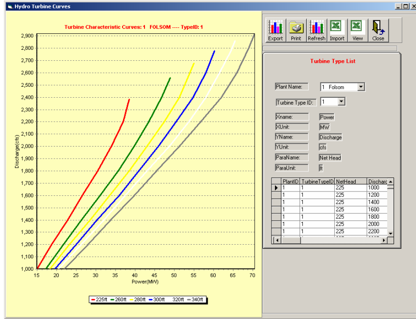
Figure F-1: Folsom Turbine Characteristic Curves (Individual Units)
